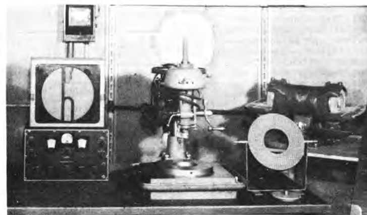
crystal testing standards used by the Signal Corps Inspection Agency in accepting crystals purchased by the Signal Corps.
